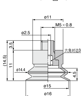
ZP2-TB15MB□□-H5
